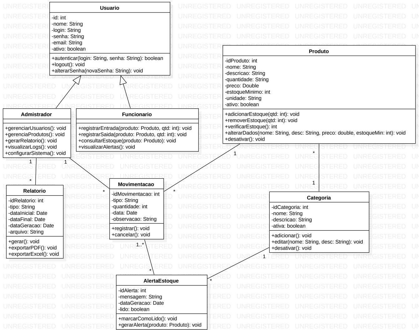
Model1::ClassDiagram1
